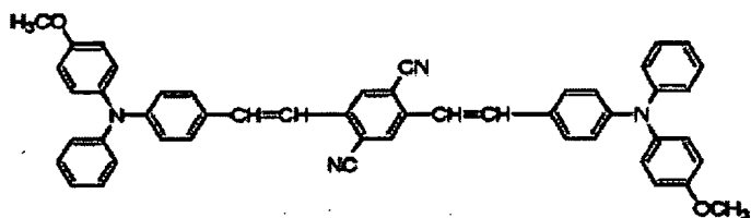
Structural formula (15)-1:
